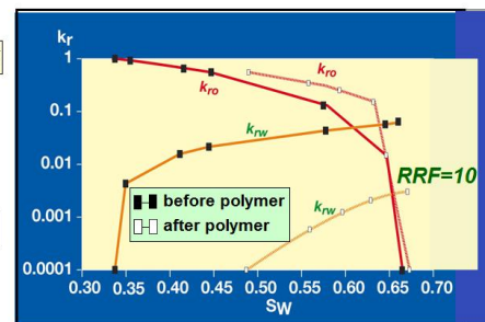
Relative permeability modification after Microgel adsorption
